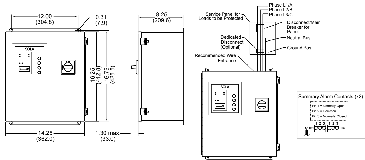
Dimensional Diagram - in. (mm)
