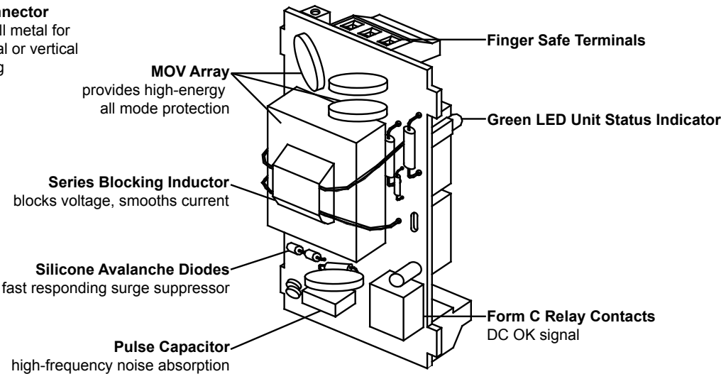
Internal View of Components
