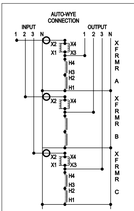
Diagram L2 – Bucking
