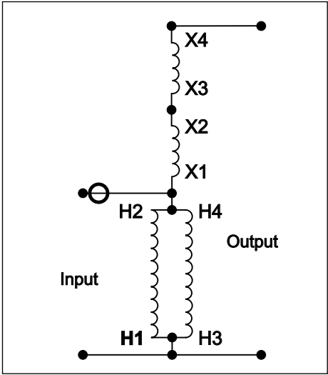
Diagram B1 – Boosting
