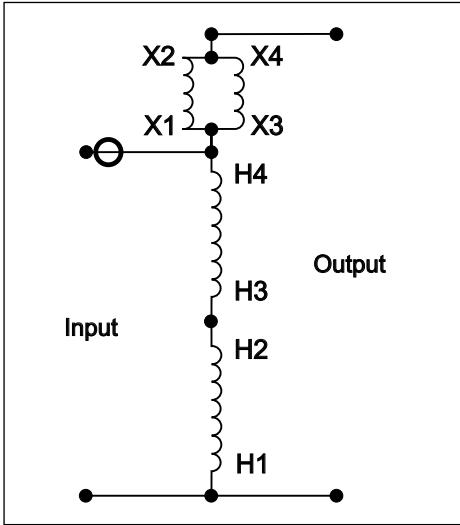
Diagram C1 – Boosting
