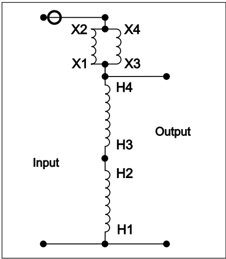
Diagram C2 – Bucking
