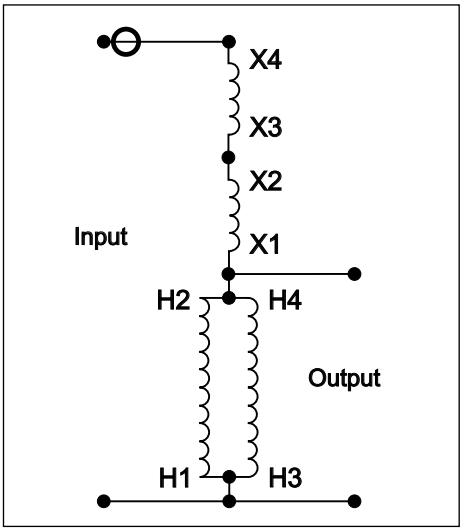
Diagram B2 – Bucking
