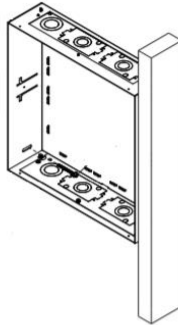
Attached to a Single Stud (25 lbs. load)
